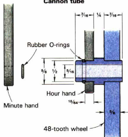
Cannon tube
