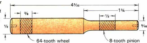
Second arbor
