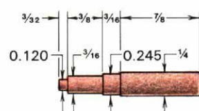
Escape-lever arbor
