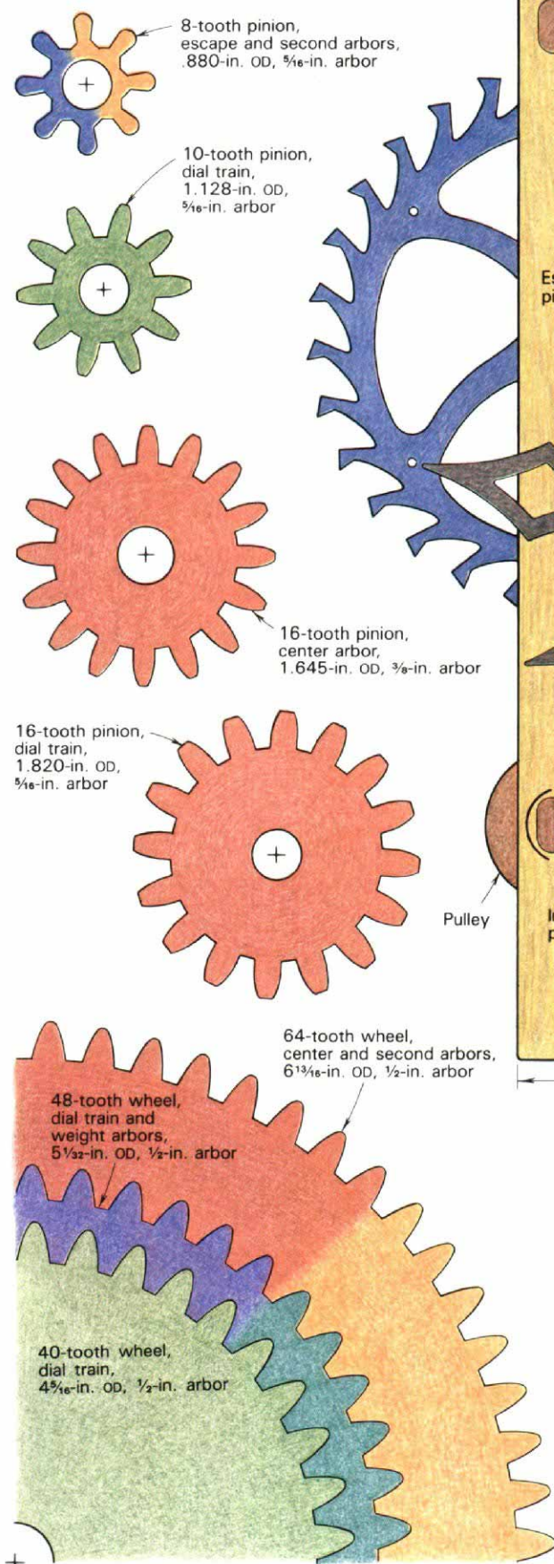
Fig. 2: Wheels, pinions and arbors
