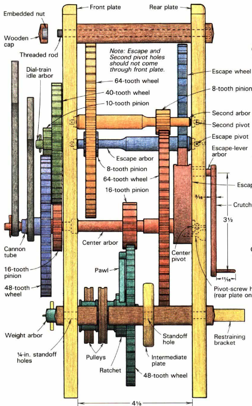
Escape arbor
