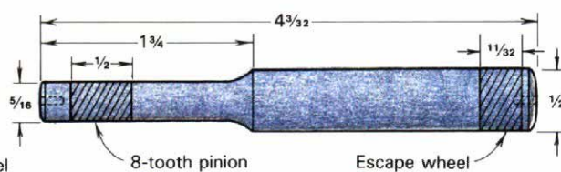
Escape arbor
