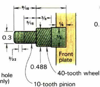
Dial-train arbor
